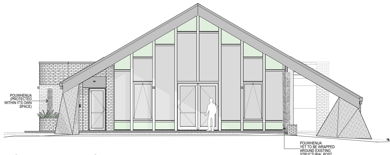
NORTH ELEVATION SCALE: 1:150 @A3
